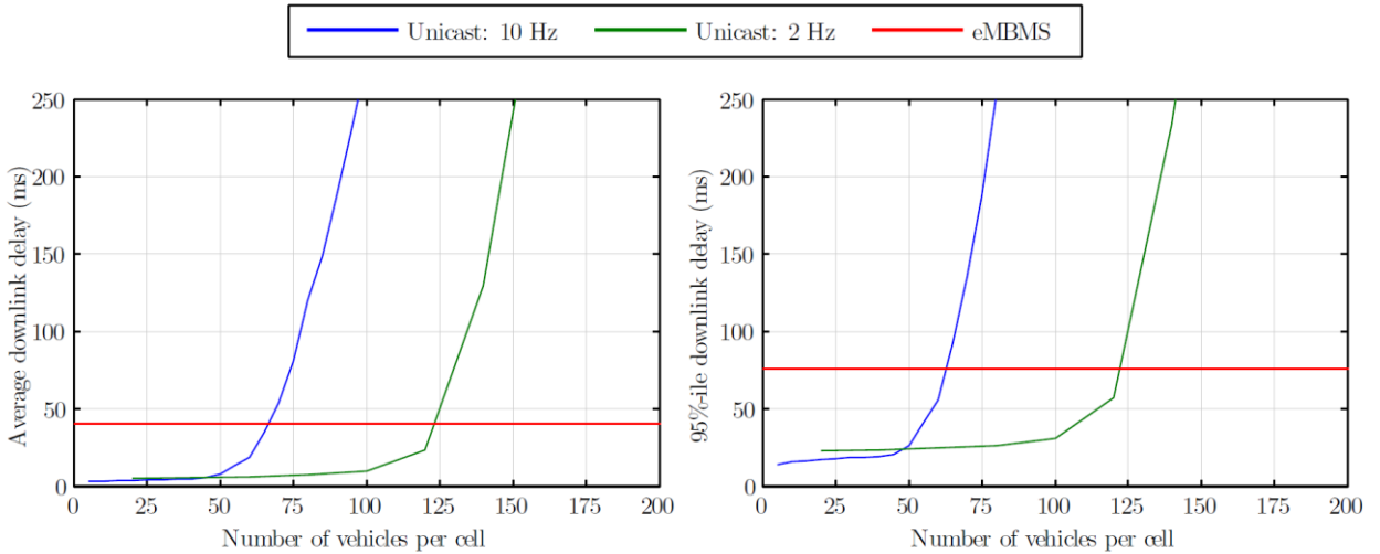
Figure 4 Downlink packet delays of CA application depending on the cell load with unicast and E-MBMS delivery modes.
