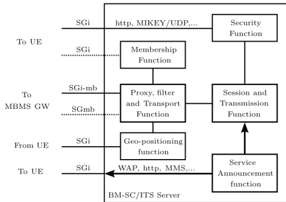
Figure 2 Main functionalities of the proposed BM-SC/ITS server node.
