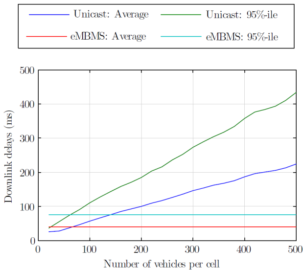
Figure 6 Downlink packet delays of RHW application depending on the cell load with unicast and E-MBMS delivery modes.
