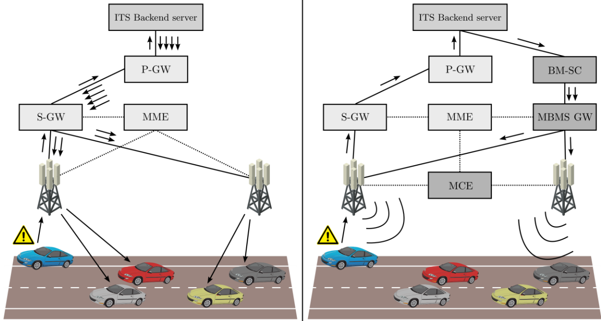
Figure 1 Unicast (left) and broadcast (right) delivery modes of a DENM over LTE cellular networks.
