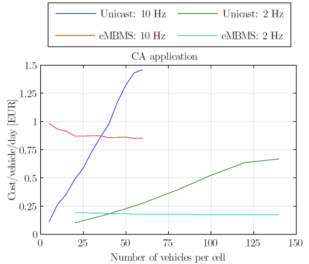
Figure 7 Cost per car and day for CA application.
