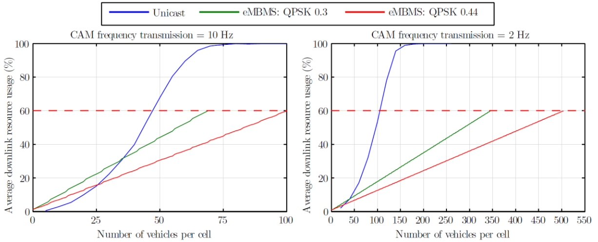
Figure 3 Downlink resource usage of CA application depending on cell load with unicast and E-MBMS delivery modes.
