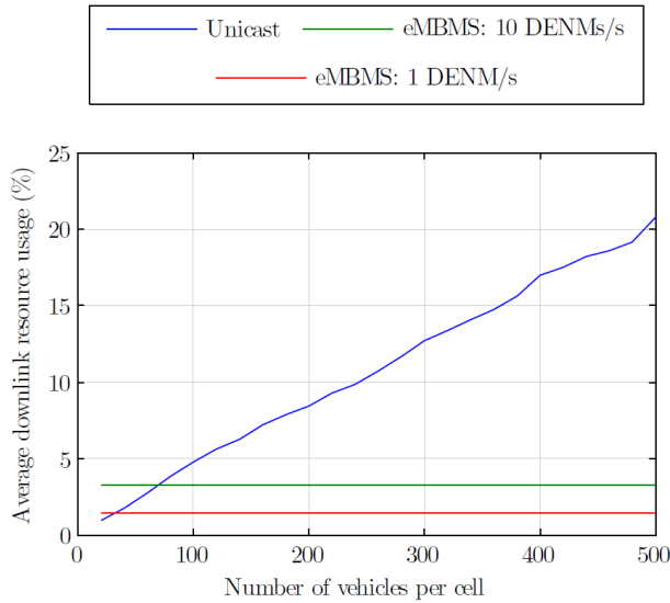
Figure 5 Downlink resource usage of RHW application depending on the cell load with unicast and E-MBMS delivery.
