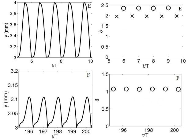
Fig. 5. Vertical coordinate (left column) and SEY impact coefficient (right column) of the effective electron for several points in Fig. 2. SEY coefficient for the impacts with the bottom (upper) wall are denoted by circles (crosses).
