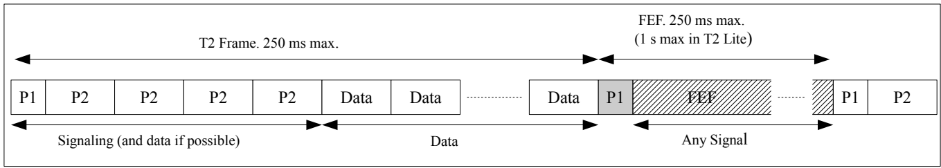
Fig. 3. T2 frame for 4K FFT size (4 P2 symbols) and FEF
