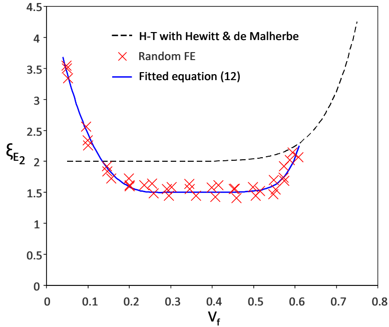
Figure 12: Plot of the expressions given in Eq. (12) fitted to the FE estimations of \xi with random distributions. Comparison with the Halpin-Tsai value ( \xi = 2 ) modified with the Hewitt and de Malherbe approximation, Eq. (3).
