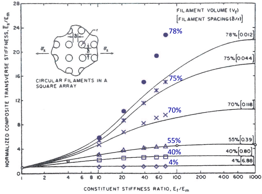
Figure 4: Square array FE estimations of E_2 computed in this work (shown with markers) superimposed on Adams and Doner's analytical solution [1, 2] .
