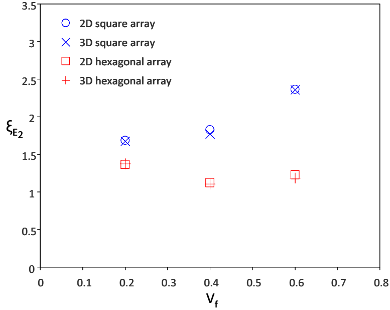
Figure 8: Sensitivity analysis to 3D effects using the models shown in Fig. 7 for three V_f (square and hexagonal arrays).
