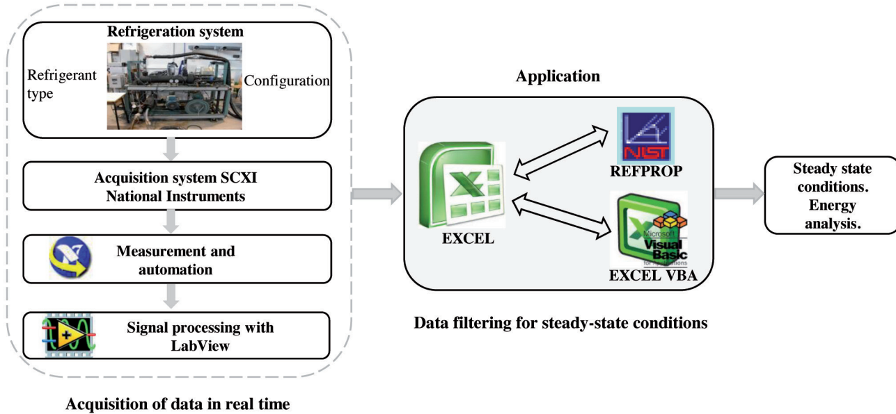
Fig. 3: General approach to develop the application
