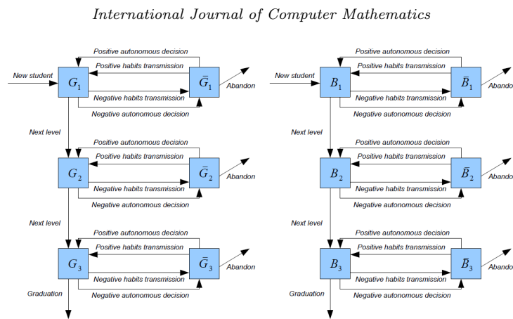
Figure 1. Flow diagram of the model (3)-(5). The boxes represent the students depending on their gender, level and academic results. The arrows denote the transit of students labelled by the cause of the flow.
