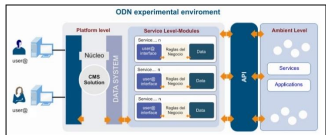
Figure 3. OpenDesigNet architecture
