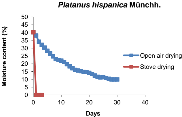
Figure 4. Drying curve for Hybrid Plane ( Platanus hispanica Münchh.)
