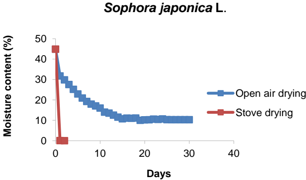
Figure 3. Drying curve for Pagoda tree ( Sophora japonica L.)
