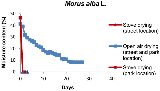
Figure 2. Drying curve for Mulberry ( Morus alba L.)
