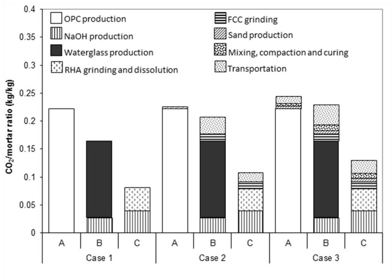
Fig. 1. Comparison of CO 2 emissions for the mortars studied in cases 1, 2 and 3.
