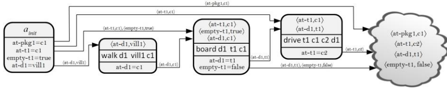
Fig. 3. Partial plan computed for the DriverLog problem example. For each action, its preconditions are shown at the top of its box and its effects at the bottom. The frontier state of the plan is displayed on the right.
