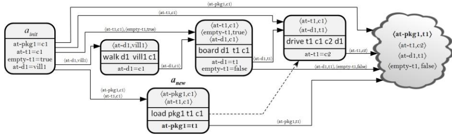
Fig. 4. Partial plan computed for the DriverLog problem example. Solid lines represent causal links and dashed lines represent orderings.
