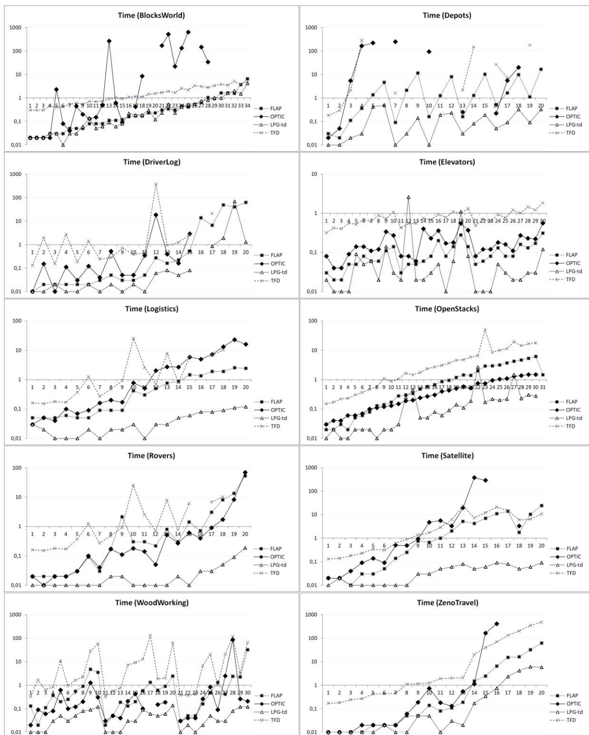
Fig. 6. Search time in second used by FLAP, OPTIC, LPG-td and TFD in the tested domains.
