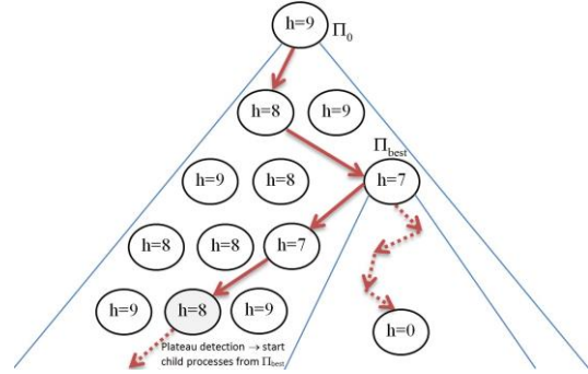
Fig. 1. Parallel A* child search started when the main search gets stuck in a plateau.
