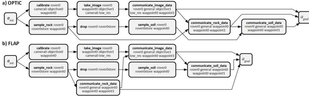
Fig. 5. Solution plan computed by a) OPTIC and b) FLAP for the second problem file of the Rovers domain.
