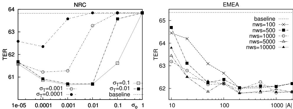
Figure 2: Effect of the different prior variance \sigma_{\mathcal{T}} and proposal variance \sigma_o (left) and number of weight quality (TER) in BPA with MCMC sampling.
