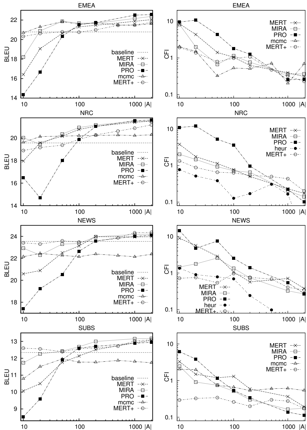
Figure 5: Performance comparison across the different corpora analysed and with the different \lambda estimation strategies. The four plots on the left display BLEU, while four plots on the right display the size of the confidence intervals.
