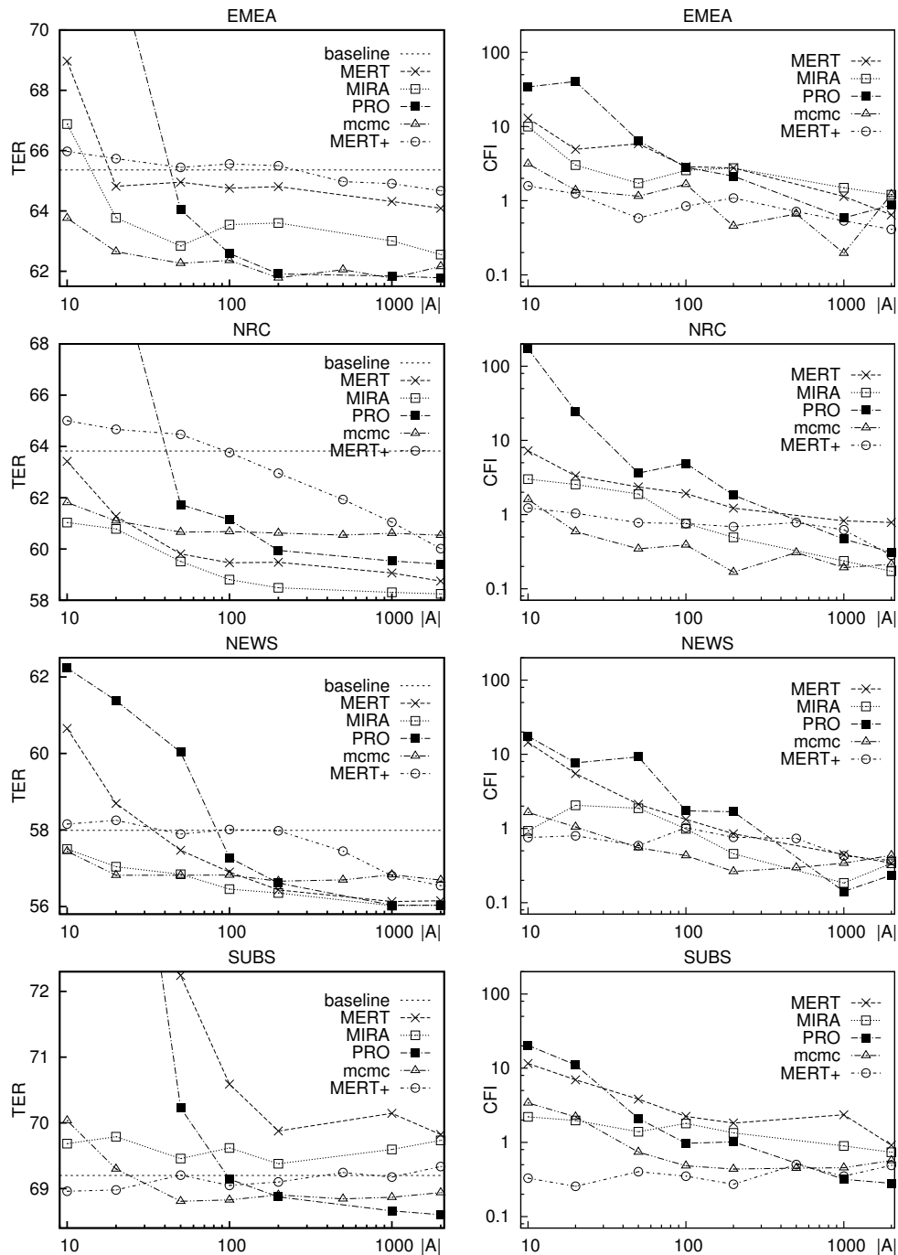
Figure 4: Performance comparison across the different corpora analysed and with the different \lambda estimation strategies. The four plots on the left display TER, while the four plots on the right display the size of the confidence intervals.
