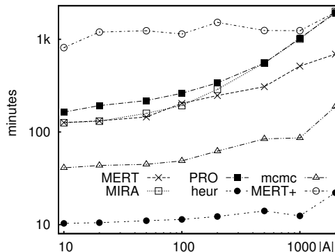
Figure 6: Time consumed by the different approaches compared. In the case of BPA, |\mathcal{S}(\lambda_{\mathcal{T}})| = 1000 and |n\text{-best}| = 500 . NRC corpus considered.
