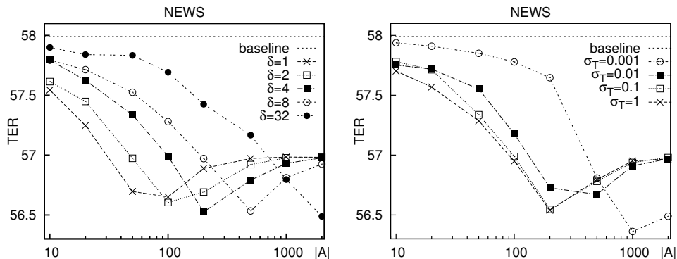
Figure 1: Effect of the \delta leveraging factor (left) and of the prior variance \sigma_{\mathcal{T}} (right) on translation quality (TER) in BPA with heuristic sampling. In the left plot, \sigma_{\mathcal{T}} = 0.1 was used. In the right plot, \delta = 4 .
