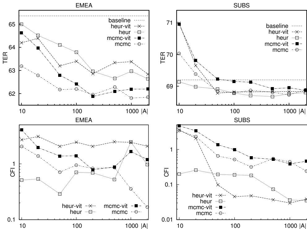
Figure 3: Batch adaptation with the Viterbi approach and different amount of adaptation set sizes. The top two plots display translation quality, while the lower two display confidence interval size.
