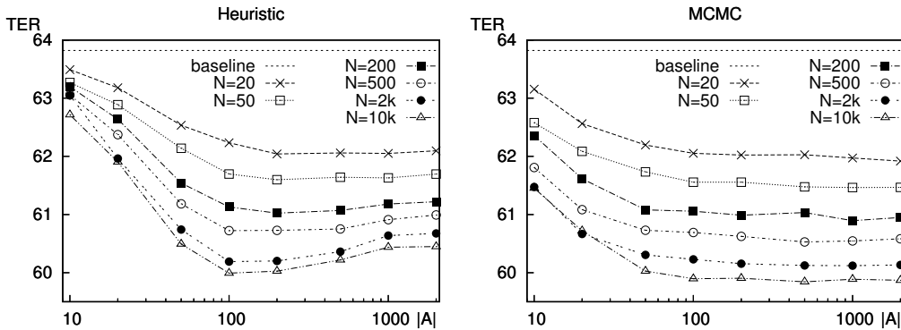
Figure 7: Translation quality with heuristic and MCMC sampling with different sizes of n -best, represented as N in the plot. NRC corpus considered.
