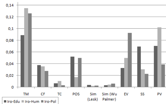
Fig. 1. Information Gain for our set of features
