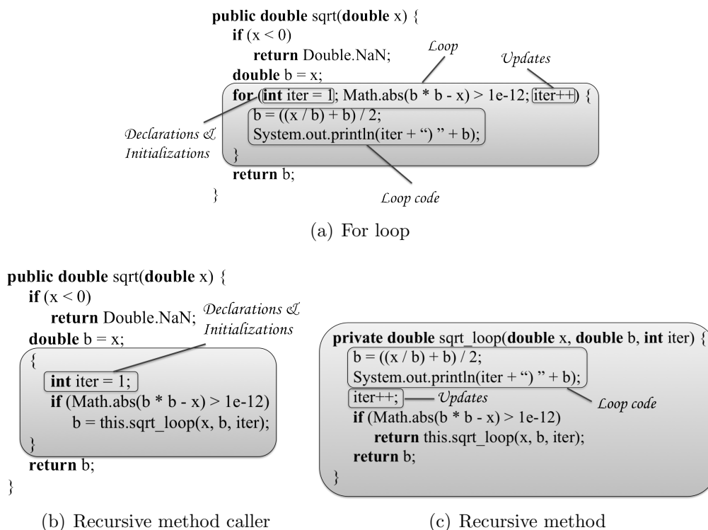
Figure 5: for-loop transformation
