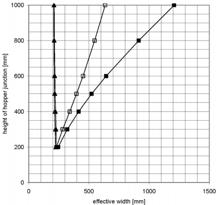
Figure 8: Effect of skirt length square: b_{,eff} at transition; triangle: b_{,eff} at h_{,cr,el} filled: support radially fixed; hollow: support radially free
