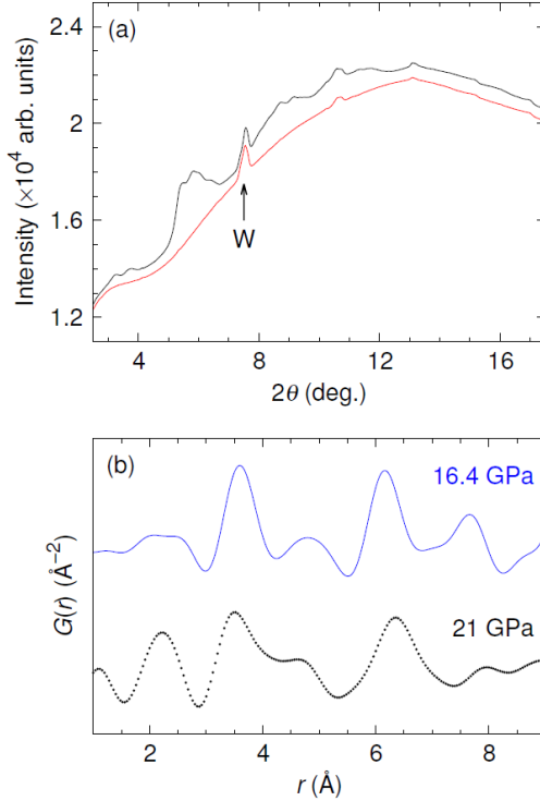
FIG. 4: (a) Diffractograms of \text{YVO}_4:\text{Eu}^{3+} nanoboxes (black solid line) and the background (red dashed line) measured at 21 GPa. The W marks the position of a reflection from the tungsten gasket (LO REESCRIBO MAS CORTO) that was unavoidable due to the divergence of the beam. (b) Calculated PDF for the scheelite-type structure of bulk \text{YVO}_4 at 16.4 GPa [15] (solid blue line) and experimental PDF for the amorphous phase of the \text{YVO}_4:\text{Eu}^{3+} nanoboxes at 21 GPa after the background correction (black dotted line).
