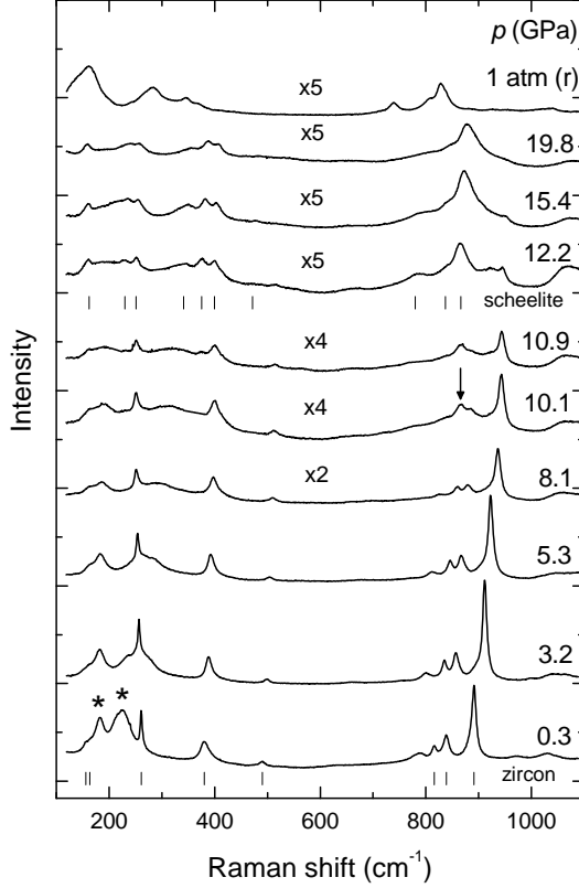
FIG. 6: Raman spectra of \text{YVO}_4:\text{Eu}^{3+} nanoboxes at different pressures. The vertical ticks show the experimental frequencies of the observed first-order Raman modes for the zircon and scheelite phases. The asterisks mark the tentatively assigned second-order modes. The vertical arrow at 10.1 GPa indicates the appearance of a Raman band attributed to the high-pressure phase. The zoom applied in each spectrum is shown.
