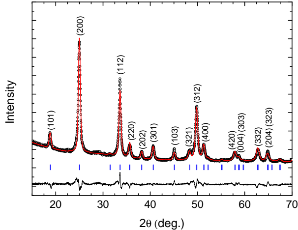
FIG. 1: X-ray diffraction pattern of \text{YVO}_4:\text{Eu}^{3+} nanoboxes at ambient conditions with the Rietveld refinement. Experimental data are plotted as empty circles and the calculated diffractogram and the residual as solid lines. The numerical values for the residuals are R_p = 2.4\% and R_{wp} = 3.2\% . Bragg reflections are indicated with vertical ticks.
