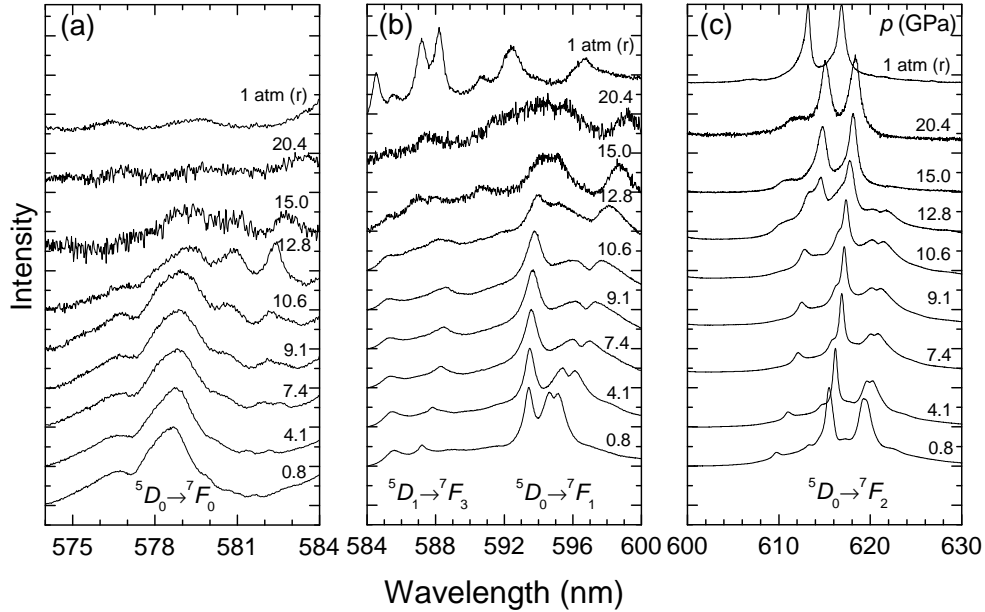
FIG. 8: \text{Eu}^{3+} photoluminescence spectra at different pressures up to 20.4 GPa showing the (a) {}^5D_0 \rightarrow {}^7F_0 , (b) {}^5D_1 \rightarrow {}^7F_3 and {}^5D_0 \rightarrow {}^7F_1 , and (c) {}^5D_0 \rightarrow {}^7F_2 normalized emission bands with respect to the most intense peak of the range.
