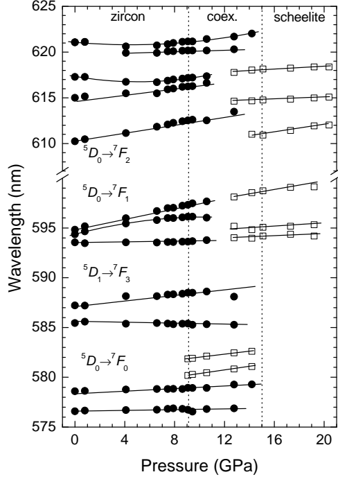
FIG. 9: Pressure dependence of the photoluminescence peak positions of \text{YVO}_4:\text{Eu}^{3+} nanoboxes. The vertical dashed lines show the onset and end of the phase transition. Solid circles and empty squares represent the electronic transitions of the low- and high-pressure phase, respectively. The solid lines are guides for the eye.
