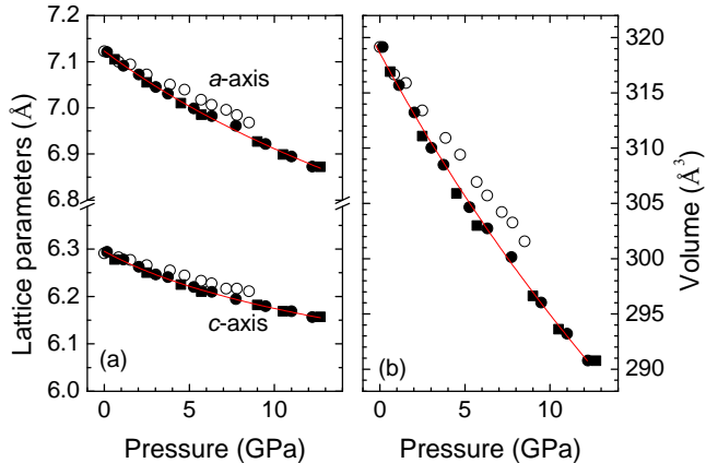
FIG. 5: (a) Pressure dependence of the lattice parameters a and c and (b) unit-cell volume V of \text{YVO}_4 . Filled circles and squares correspond to data of nano \text{YVO}_4:\text{Eu}^{3+} obtained in run1 and run2, respectively. Empty circles correspond to data for bulk \text{YVO}_4 reported by Wang et al. [15]. Continuous lines are the Murnaghan and second-order Birch-Murnaghan equations of state fits to the lattice parameters and volume, respectively.
