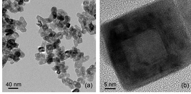
FIG. 2: (a) TEM micrograph of a group of \text{YVO}_4:\text{Eu}^{3+} nanoboxes and (b) HRTEM micrograph a single nanoparticle.
