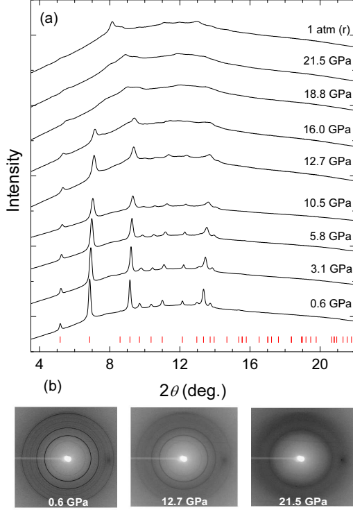
FIG. 3: (a) Selection of X-ray diffractograms of \text{YVO}_4:\text{Eu}^{3+} nanoboxes at different pressures from run2. Vertical ticks at 0.6 GPa indicate the Bragg reflections. (b) Image plate shots at three different pressures showing the evolution of the X-ray diffraction rings along the amorphization of \text{YVO}_4:\text{Eu}^{3+} .
