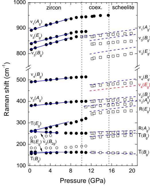
FIG. 7: Pressure dependence of the experimentally observed first-order (solid circles) and second order (empty circles) Raman active modes of the low-pressure and high-pressure (empty squares) phases of \text{YVO}_4:\text{Eu}^{3+} nanoboxes. For comparison, the fits for bulk \text{YVO}_4 (solid and dashed blue lines) are also given [16]. The red dashed line shows the \nu_4(E_g) mode not detected in our experiment with \text{YVO}_4:\text{Eu}^{3+} nanoboxes, but present in the bulk. The vertical black dashed lines represent the onset and end of the phase transition. \nu_i stands for the internal modes of the \text{VO}_4 molecule and R and T represent the pure rotation and translation of the \text{VO}_4 molecule [16].
