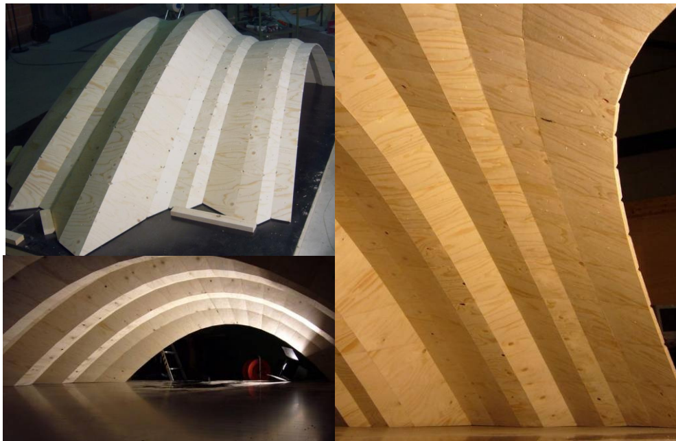
Figure 3: Shell structures made out of timber block panels
