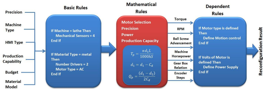
Figure 5. Flow of data and processing through three steps of rules defined.
