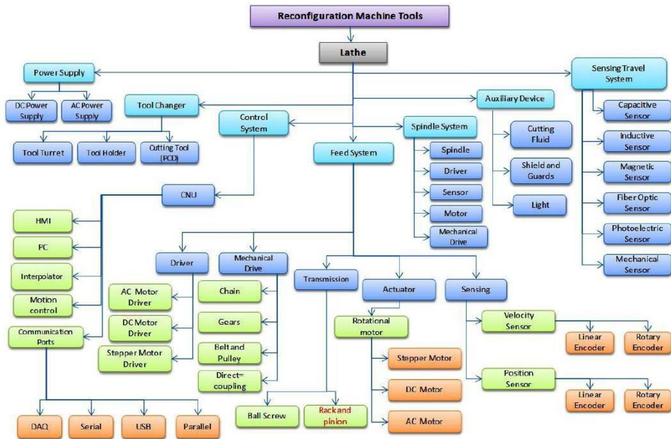
Figure 4. Tree diagram of the components and subcomponents of a lathe.
