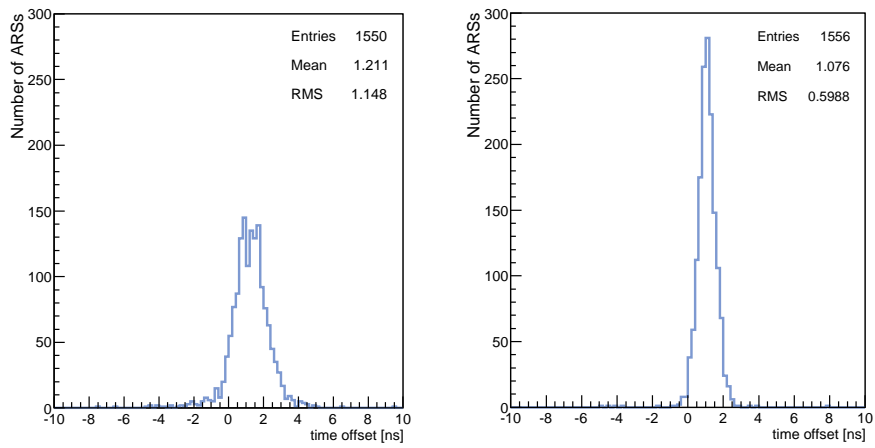
Figure 10: Distribution of the ARS timing corrections after one iteration (left) and after five iterations (right) of the muon time residuals method. The increase in the number of entries is due to a few ARS which are outside the time range in the left figure.
