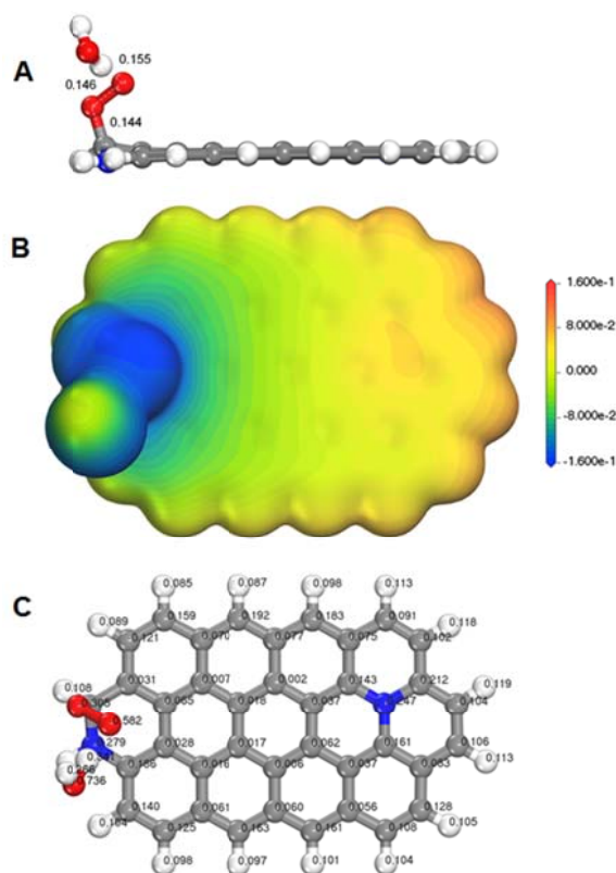
Figure 3. Monodentate chemisorbed state of molecular oxygen on the carbon atom a of the configuration displayed as Fig. 1C. An explicit water molecule in addition to a continuum model was used as solvation effect treatment. (A) Adsorbent-adsorbate-solvent geometry (distances in nm). (B) Electrostatic potential in Ha/e - mapped on the electron isodensity surface \rho = 10 \text{ e}^- \text{ nm}^{-3} . (C) Mulliken partial charges in e - .
