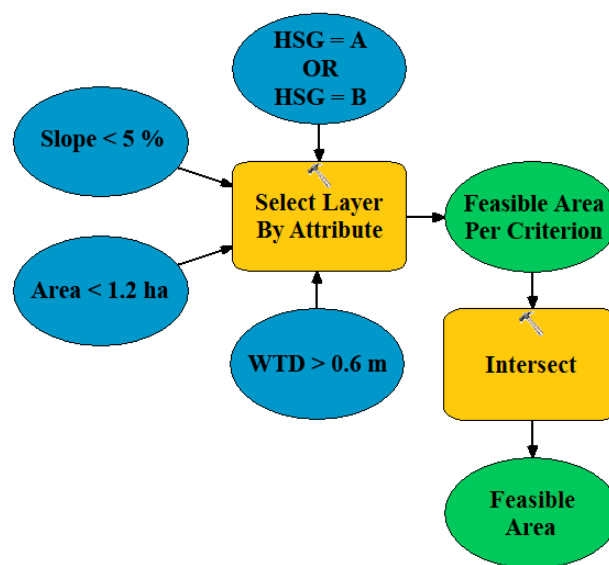
Figure 1. Workflow for the identification of feasible areas for the implementation of Permeable Pavement Systems (PPS).
