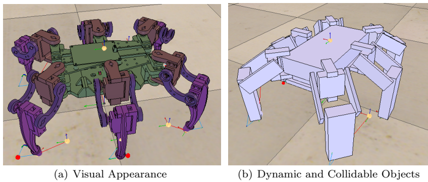
Fig. 3 Simulation of HF08 hexapod robot in V-REP.
