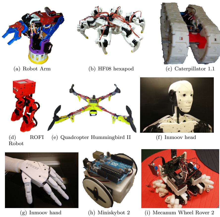
Fig. 1 Examples of free printable robots. From left to right and top to bottom: Robot Arm [5], Hellium From HF08 Hexapod Robot [26], Caterpillator 1.1 [24], ROFI Robot Five [9], Quadcopter Hummingbird II [19], Inmoov head and hand [20], Miniskybot2 [14], Mecanum Wheel Rover 2 [21].
