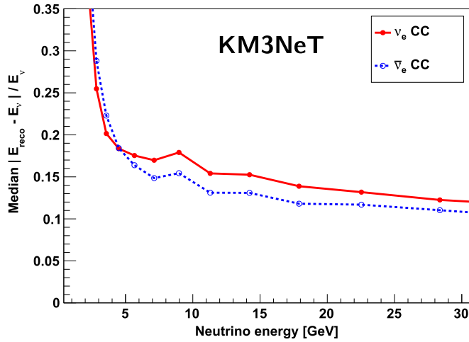
Figure 86. Median fractional energy resolution ( |E_{reco} - E_\nu|/E_\nu ) as a function of neutrino energy for \nu_e CC (red) and \bar{\nu}_e CC (blue) events weighted according to the Bartol flux model.
