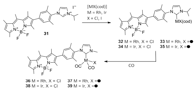
Scheme 9 Synthesis of the bimetallic complexes 32-35 and their reaction with CO.
