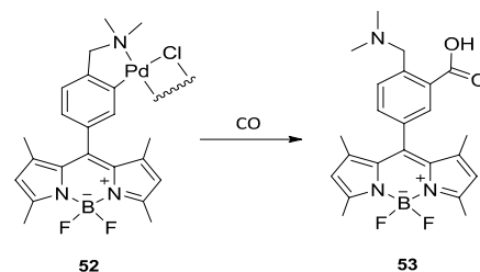
Scheme 13 Reactivity of the palladium complex 52 with CO.
