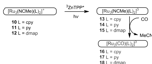
Scheme 4 The reaction of trinuclear ruthenium complexes with CO.
