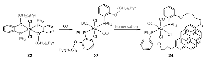
Scheme 7 Reactivity of the ruthenium complex 22 with CO.
