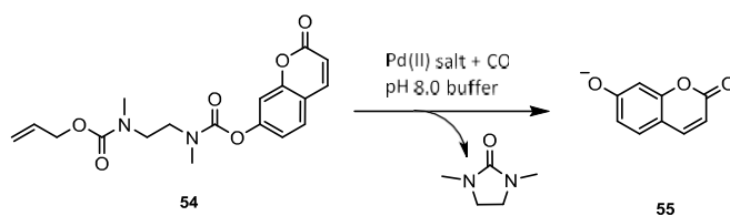
Scheme 14 Reactivity of 54 with CO to give fluorescent 55 .
