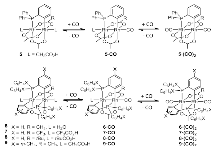
Scheme 3 Binuclear rhodium complexes 5-9 and the corresponding products obtained upon coordination of one and two molecules of CO in the axial positions.
