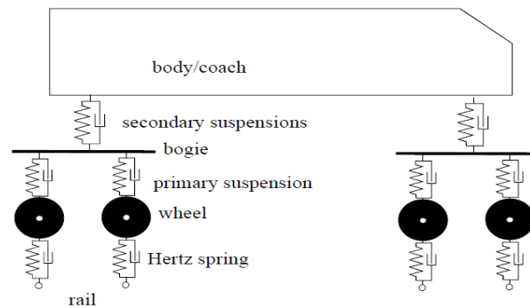
Fig. 2 - Vehicle model used in the simulation.
