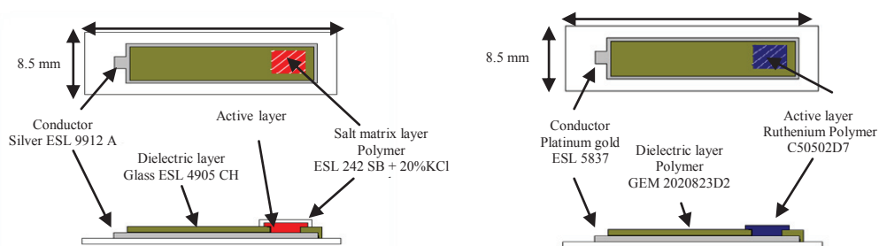
Fig. 1. Cross-sections of Thick-Film reference electrode (left) and pH ion selective electrode (right)
