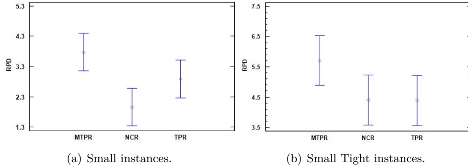
Figure 3: Means Plot and LSD intervals at the 95% confidence level for the algorithms with local search (Small and Small Tight instances).
