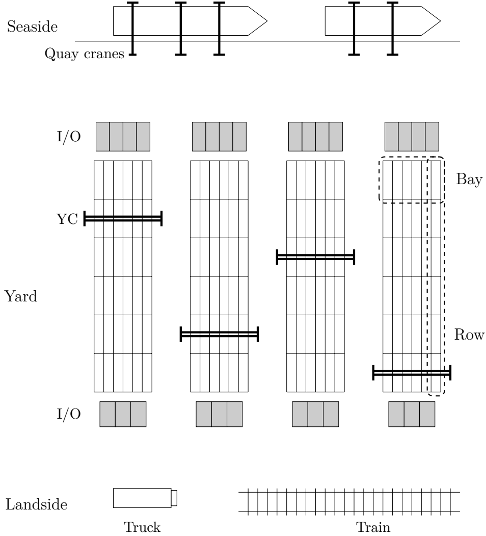
Figure 1: Top view of an automated terminal
