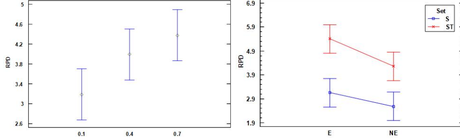
(a) Means Plot for RPD and R_j factor. (b) Interaction plot (Set and W_j ). Small instances (Algorithms with LS). instances (Algorithms with LS).
